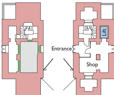
Ground-floor plan
