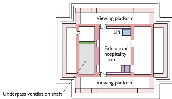
Gallery-floor plan
