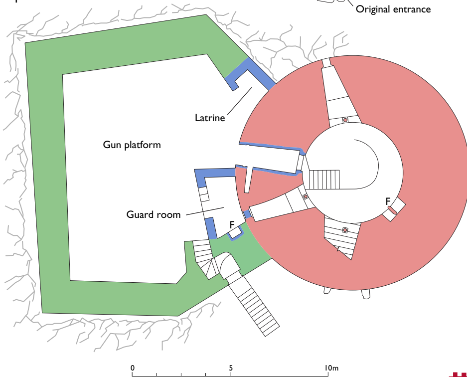
Ground-floor plan
